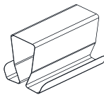
移动白板纸夹 Paper Clip For mOVEABLE White BOARD W60*D46*H38
